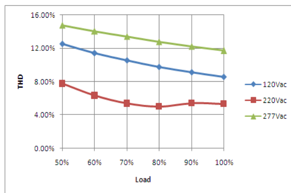
THD Curve
