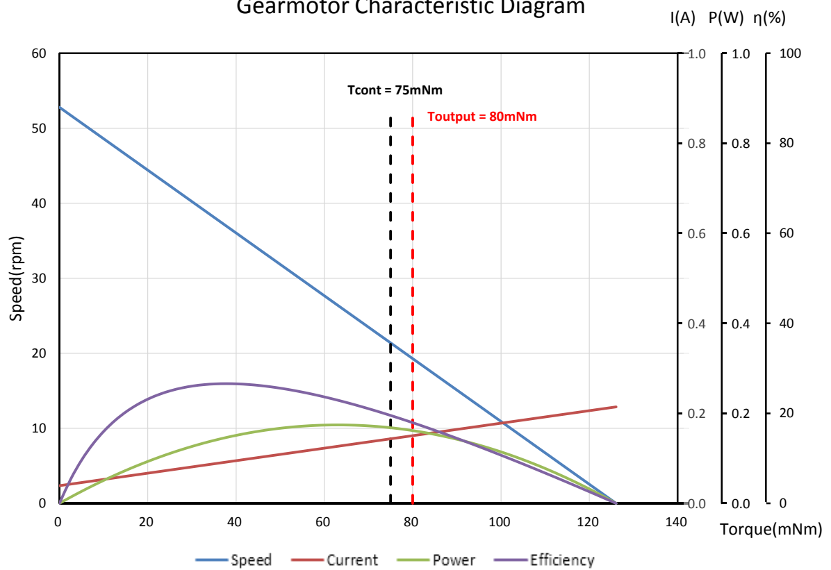
Gearmotor Characteristic Diagram
