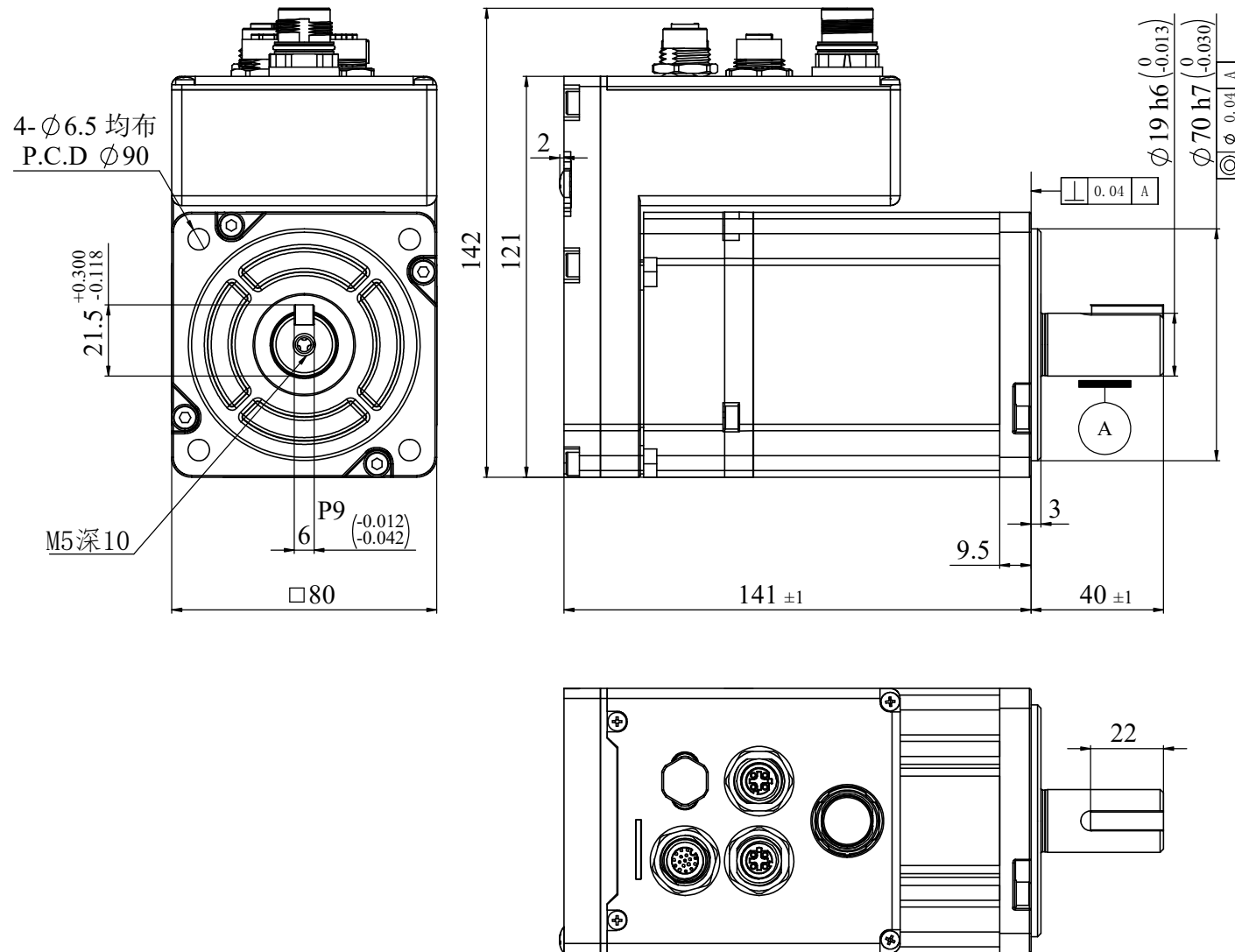
MDXT82GNBIPA000 尺寸图 MDXT82GNBIPA000 2D drawing
